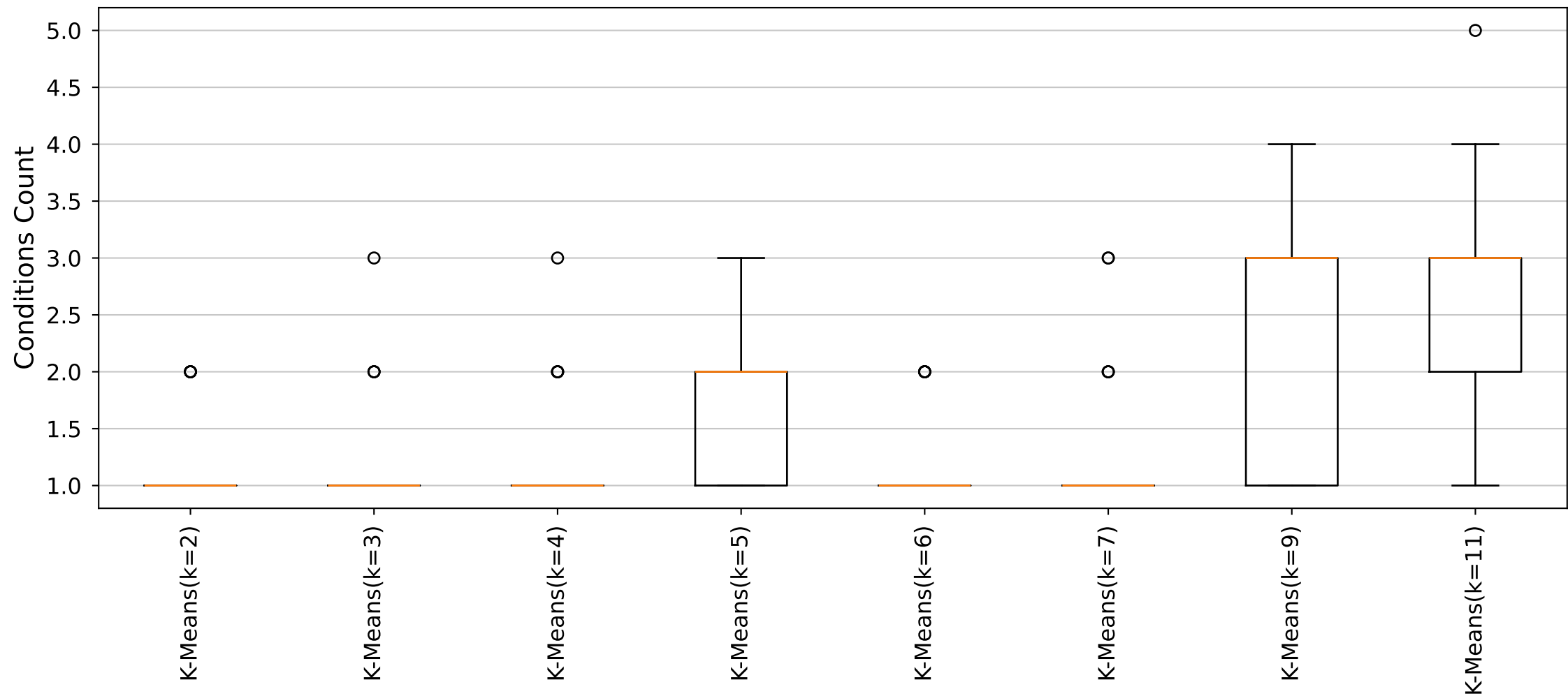
YARA Rules Conditions Count Distribution (Cluster9_Size11 dataset)
